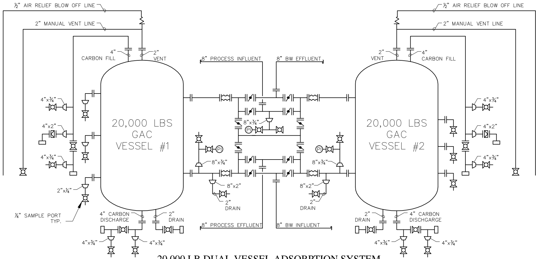
20,000 LB DUAL VESSEL ADSORPTION SYSTEM
